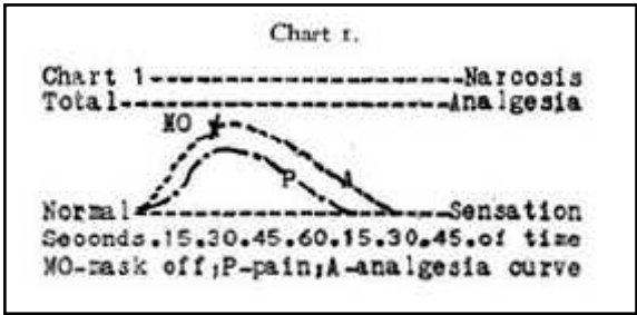
Figure 1: Guedel's labor analgesia with the nitrous oxide technique. On the x axis is time in 15-second increments. Pure nitrous oxide is inhaled from the beginning of the contraction until the black star initialed MO (mask off). Note that the analgesia curve stays above the pain curve for the duration of the contraction. In Guedel's papers, there are several variations on this chart, depending on the rapidity of the pain at onset, the duration of the contraction, and patient characteristics.
